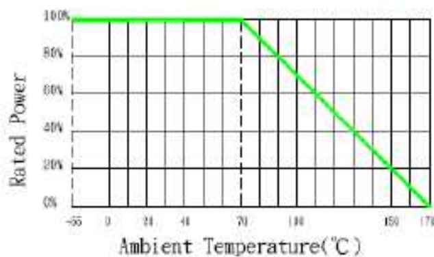
Operating Temperature Range: -55 to +170 deg.C
